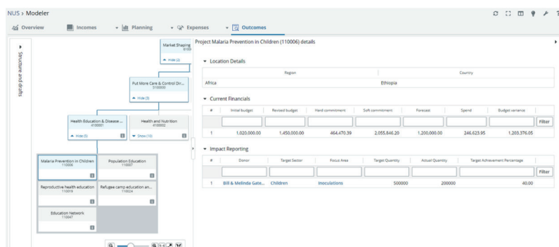
Figure 1.3 Outcomes Modelling
